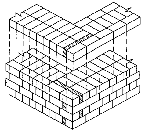
ISOMETRIC VIEW OF TWO BRICK WALL
