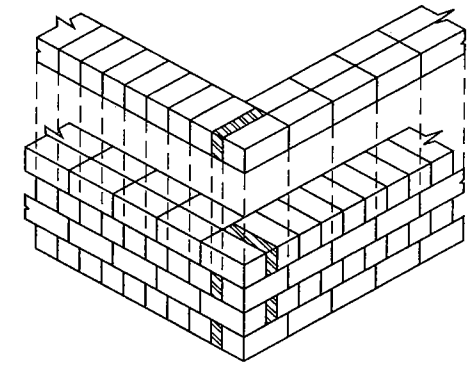
ISOMETRIC VIEW OF ONE BRICK WALL
