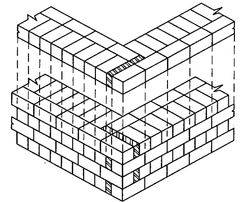
ISOMETRIC OF ONE AND A HALF BRICK WALL
